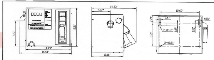
Separated nozzle holder provided with pump start/ stop lever
